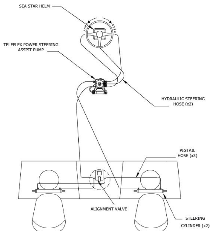
Optional steering system on 235CC, with power steering pump.
