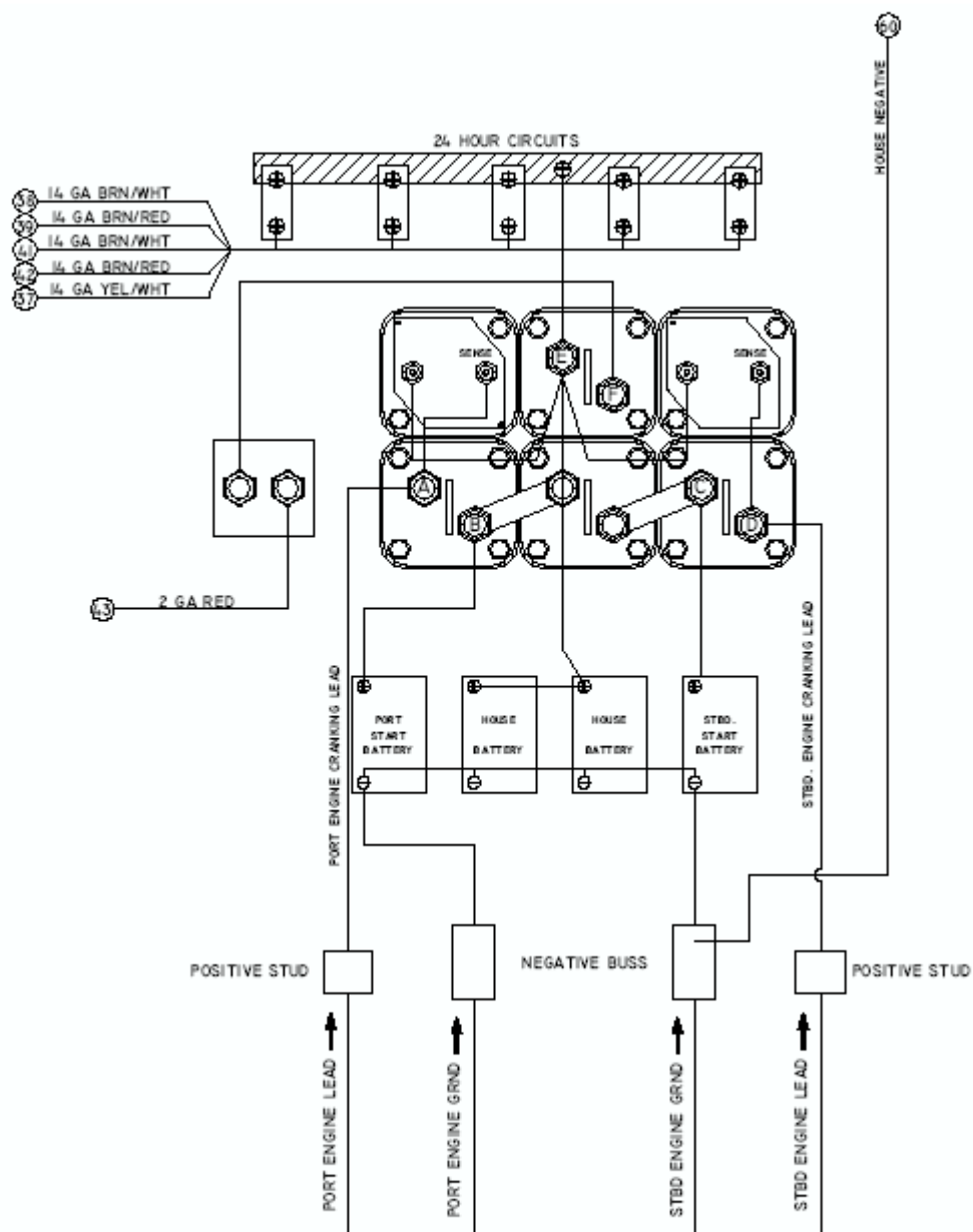
BATTERY MANAGEMENT SYSTEM DIAGRAM
