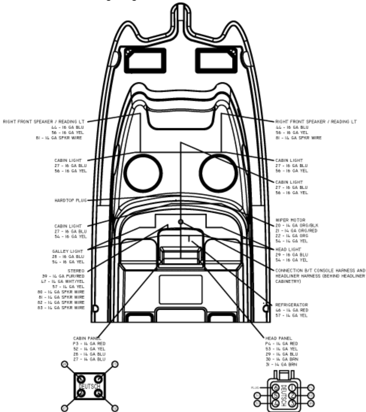
HARDTOP PLUG
